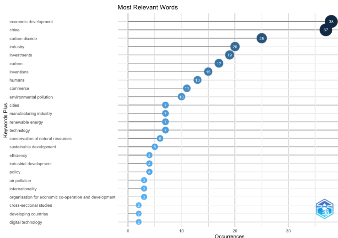
Figure 14: Keywords
