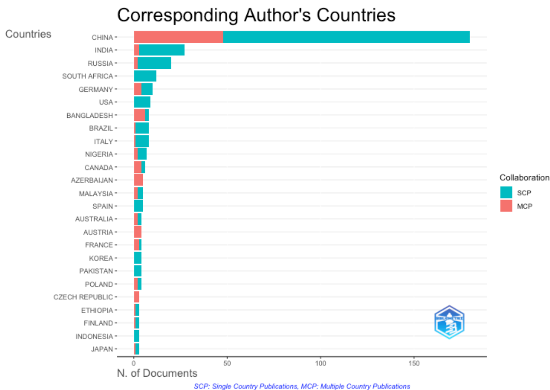
Figure 9: Authors Countries
