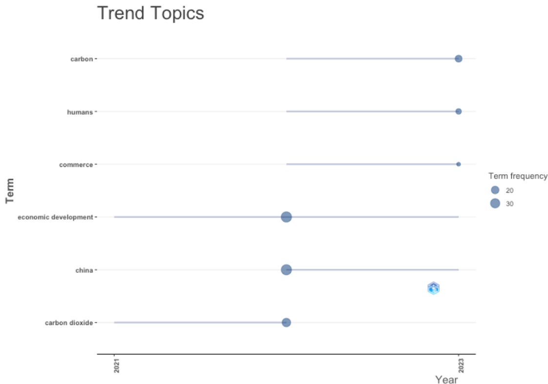
Figure 17: Topic Trends
