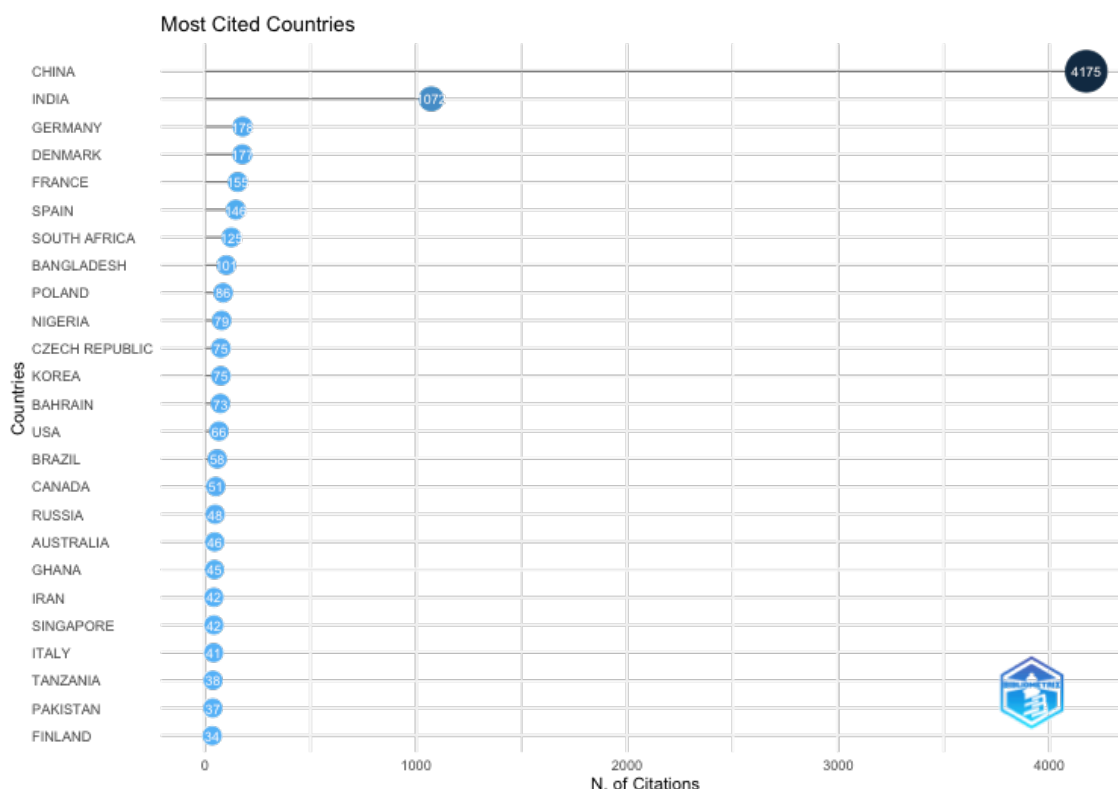
Figure 12: Country's Citation
