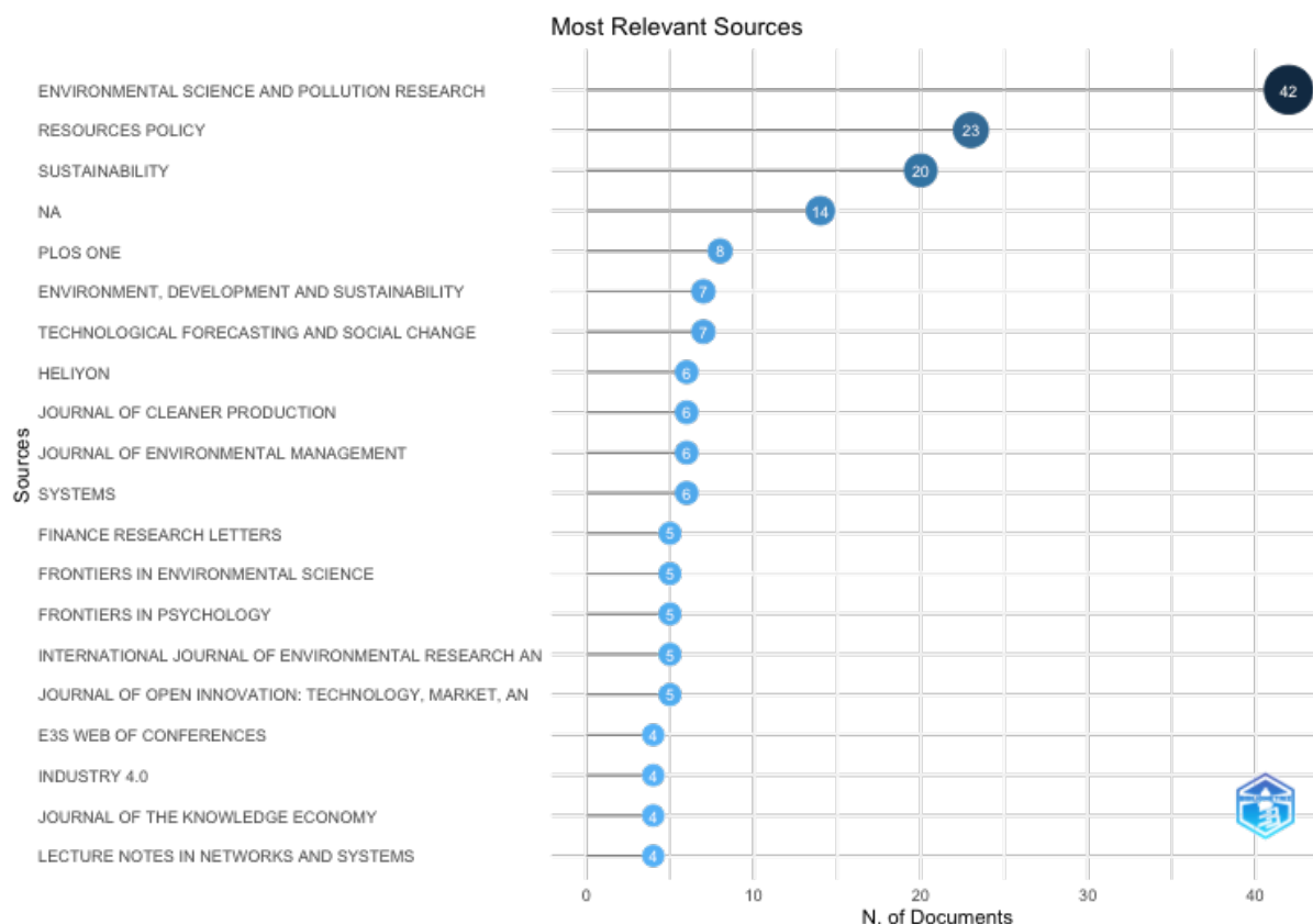
Figure 3: Relevant Sources
