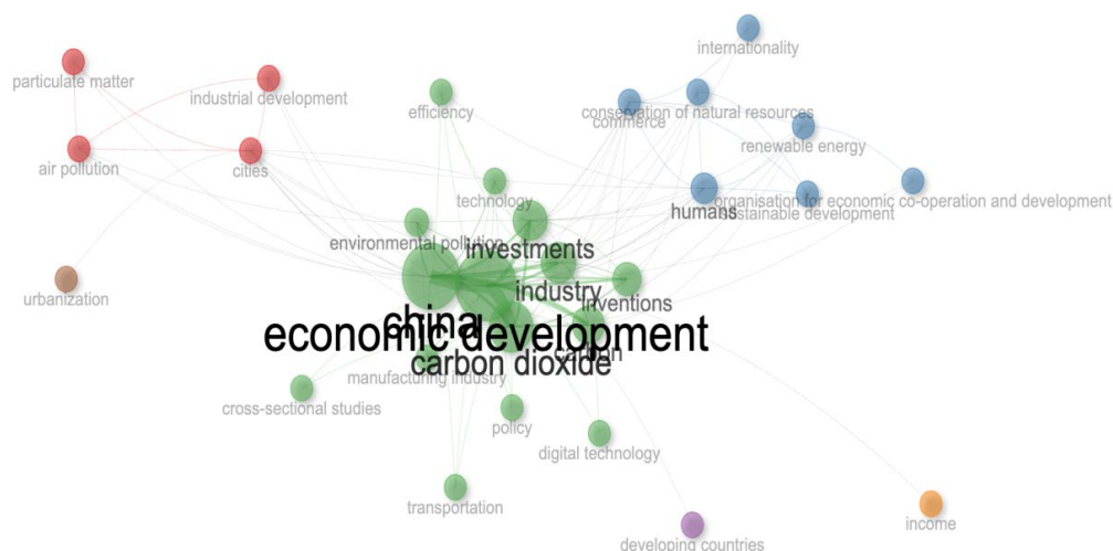
Figure 17: Topic Trends
